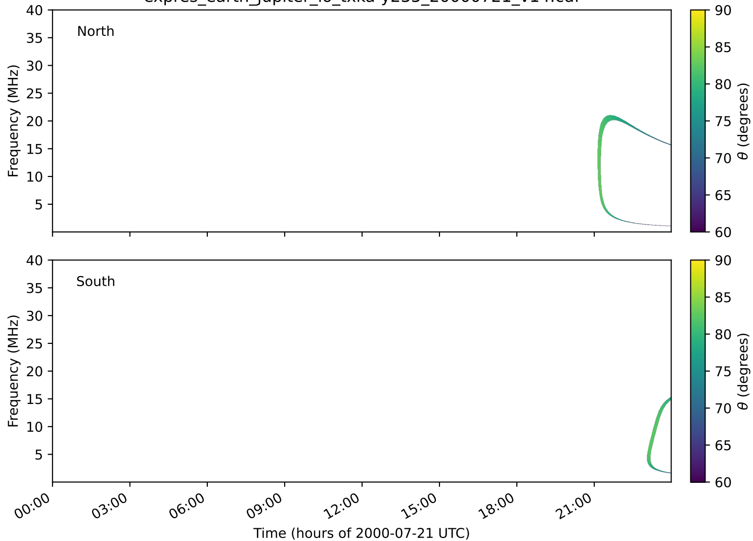
expres_earth_jupiter_io_txka-y235_20000721_v14.cdf
