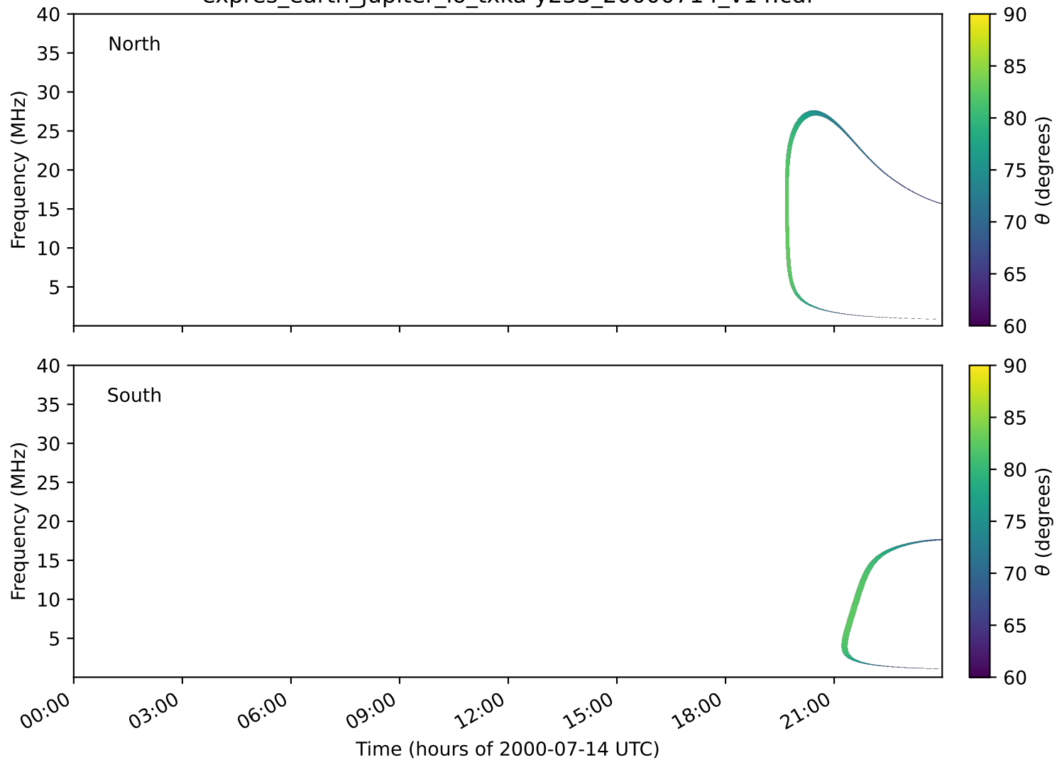
expres_earth_jupiter_io_txka-y235_20000714_v14.cdf
