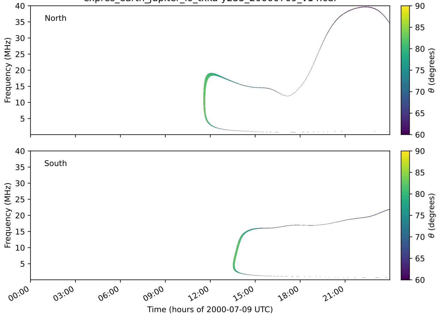
expres_earth_jupiter_io_txka-y235_20000709_v14.cdf
