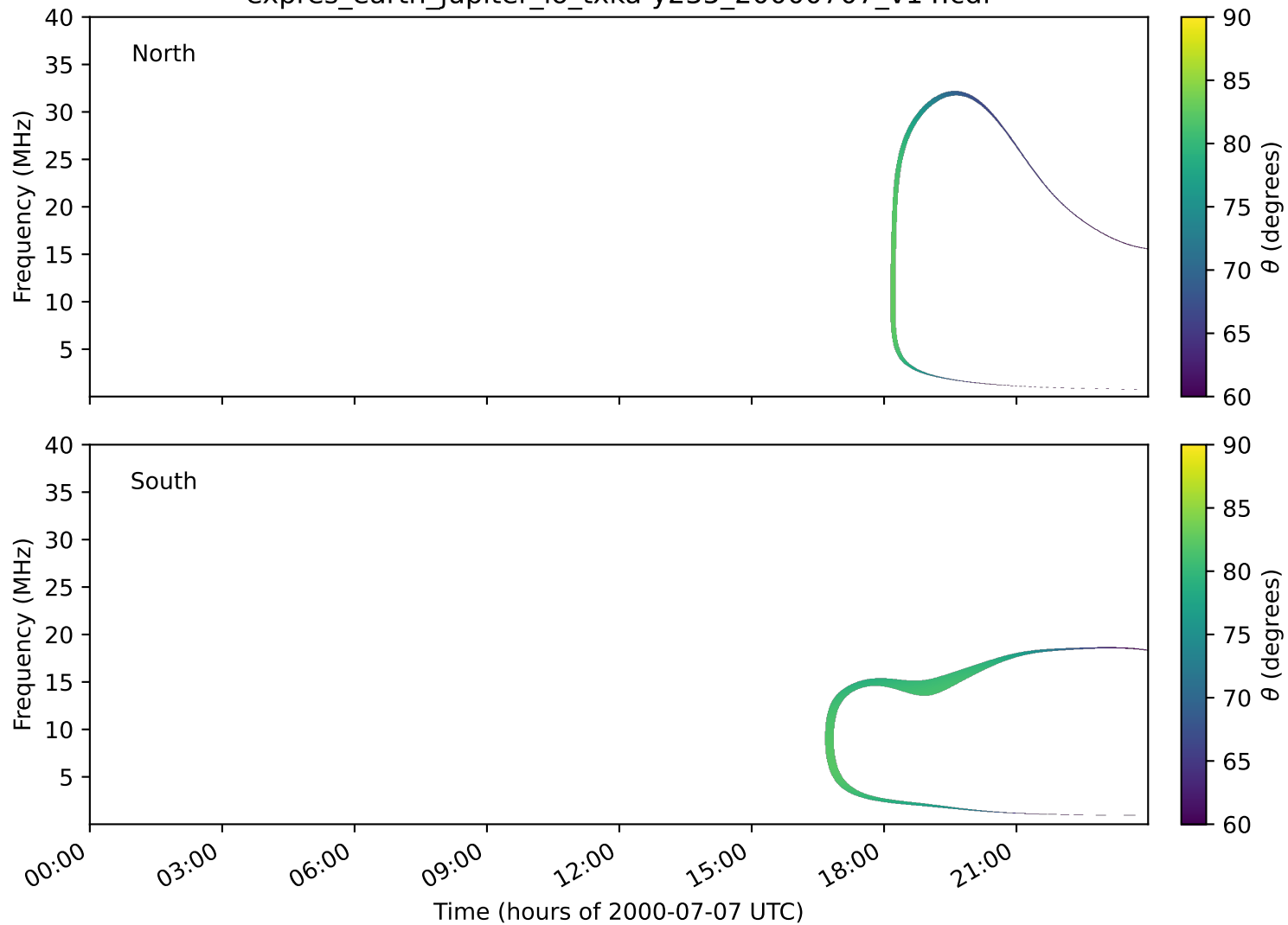
expres_earth_jupiter_io_txka-y235_20000707_v14.cdf
