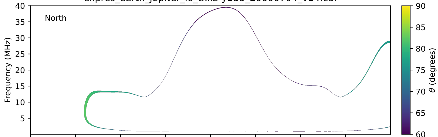
expres_earth_jupiter_io_txka-y235_20000704_v14.cdf
