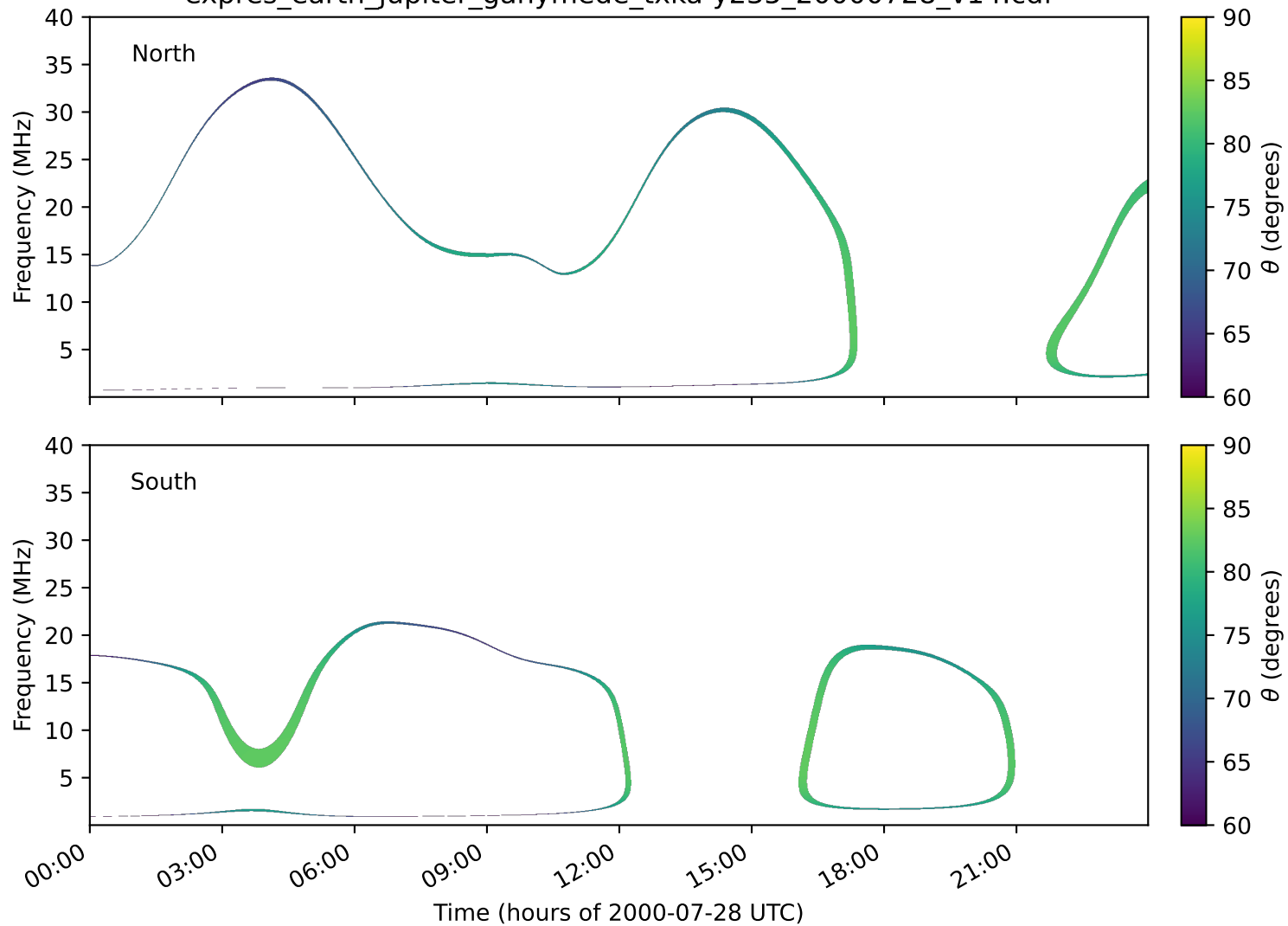
expres_earth_jupiter_ganymede_txka-y235_20000728_v14.cdf
