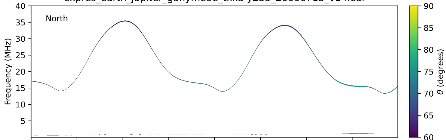
expres_earth_jupiter_ganymede_txka-y235_20000713_v14.cdf
