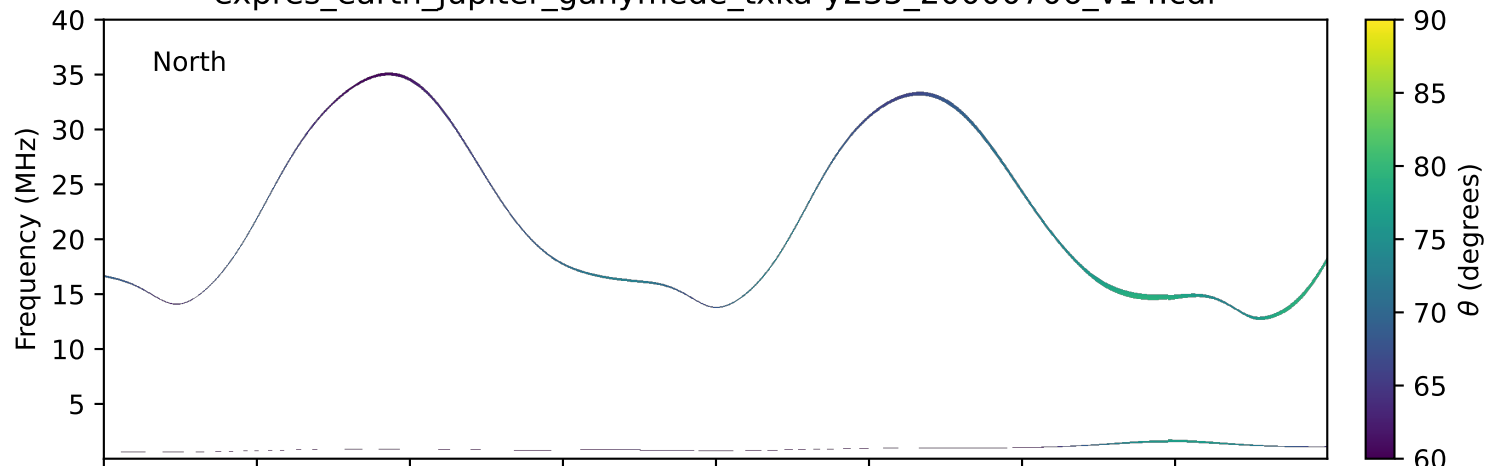
expres_earth_jupiter_ganymede_txka-y235_20000706_v14.cdf
