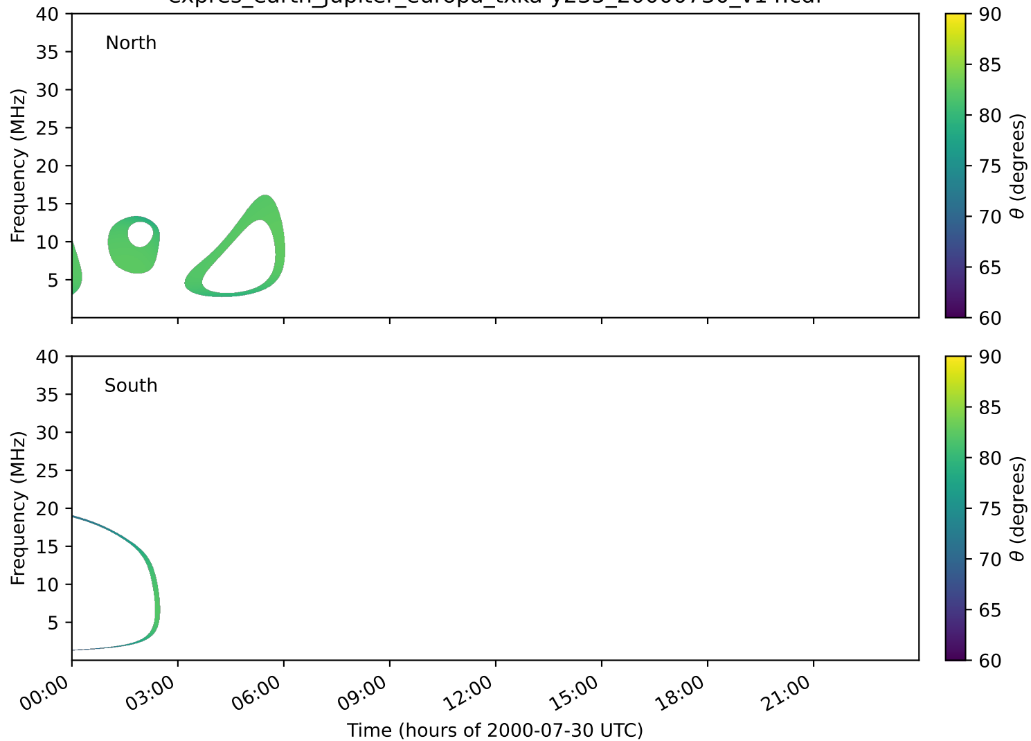
expres_earth_jupiter_europa_txka-y235_20000730_v14.cdf
