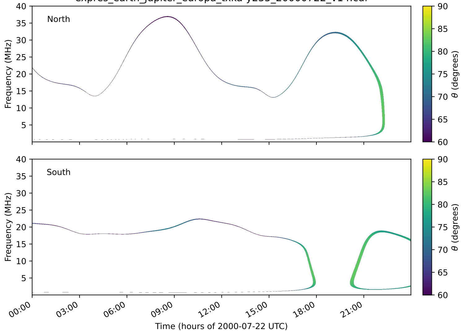
expres_earth_jupiter_europa_txka-y235_20000722_v14.cdf
