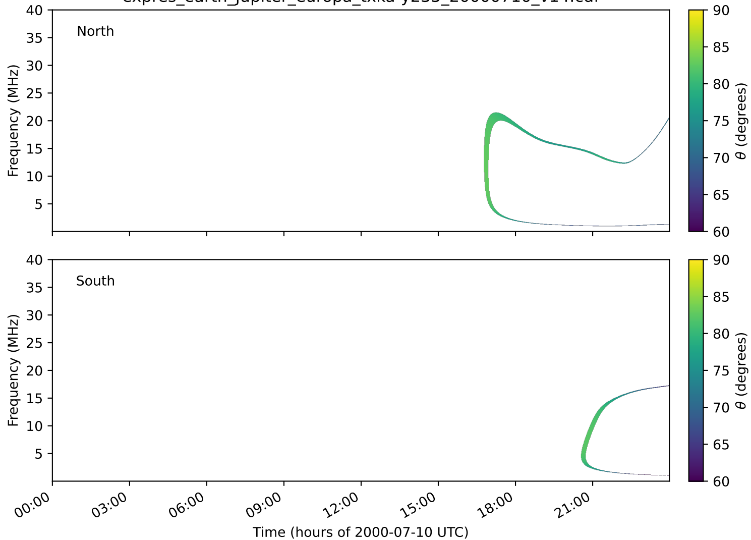
expres_earth_jupiter_europa_txka-y235_20000710_v14.cdf
