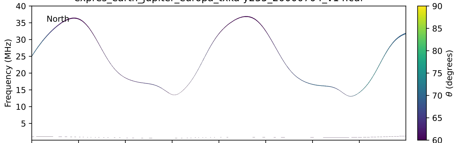
expres_earth_jupiter_europa_txka-y235_20000704_v14.cdf
