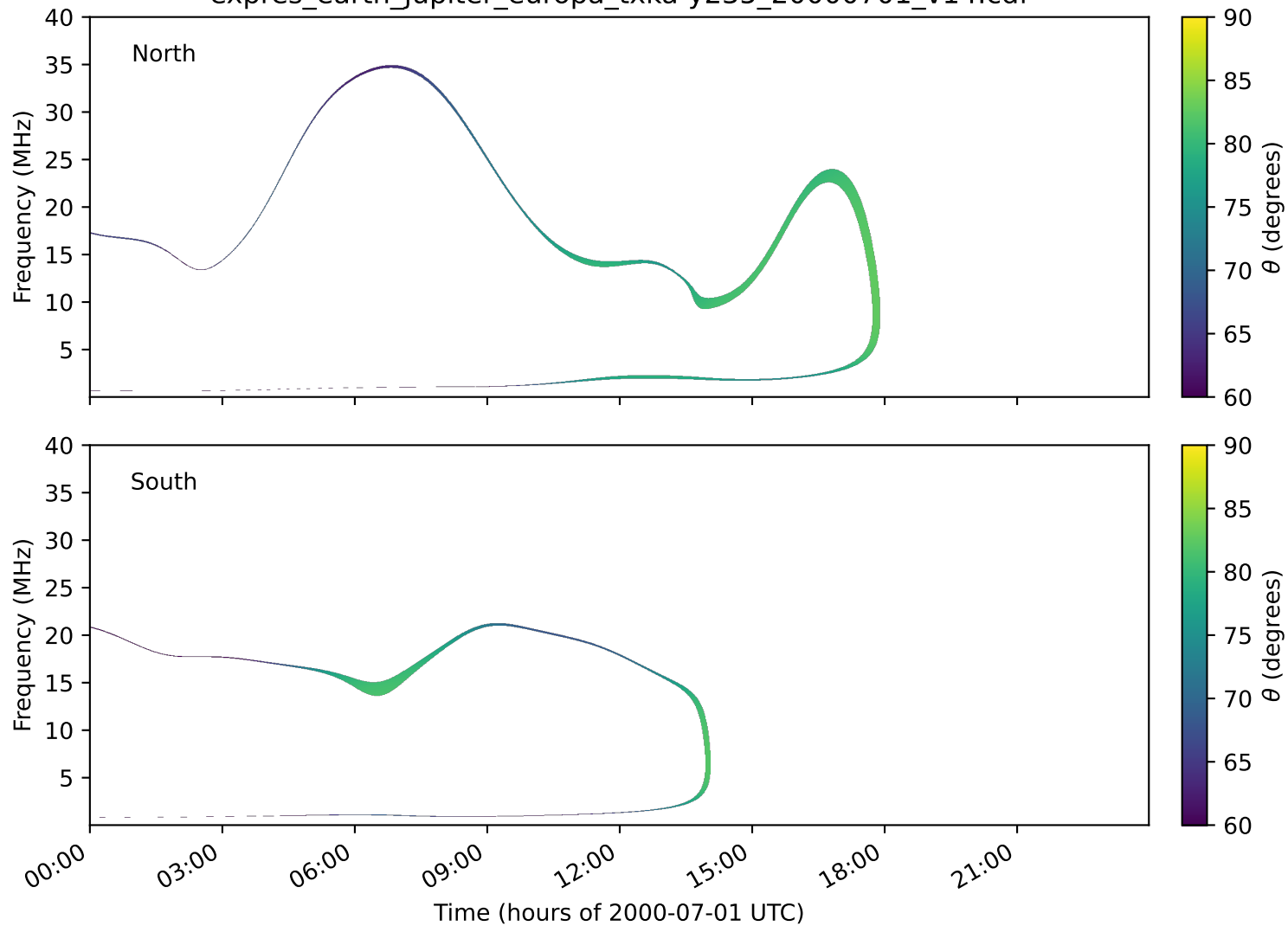
expres_earth_jupiter_europa_txka-y235_20000701_v14.cdf
