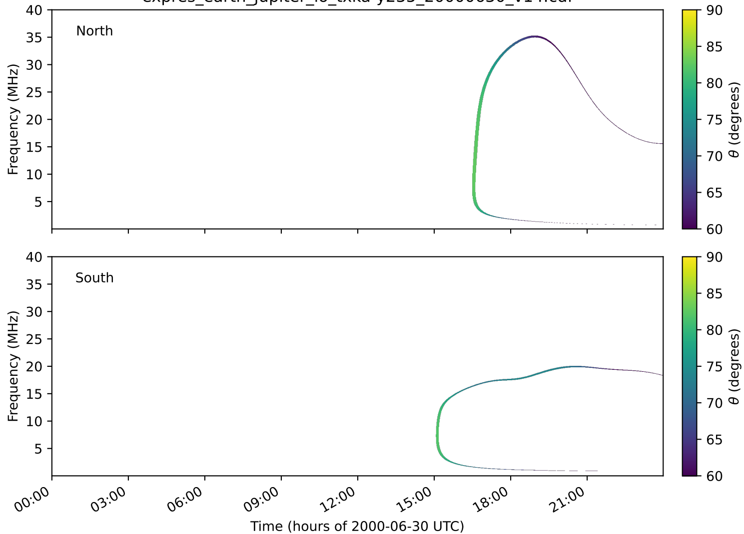
expres_earth_jupiter_io_txka-y235_20000630_v14.cdf
