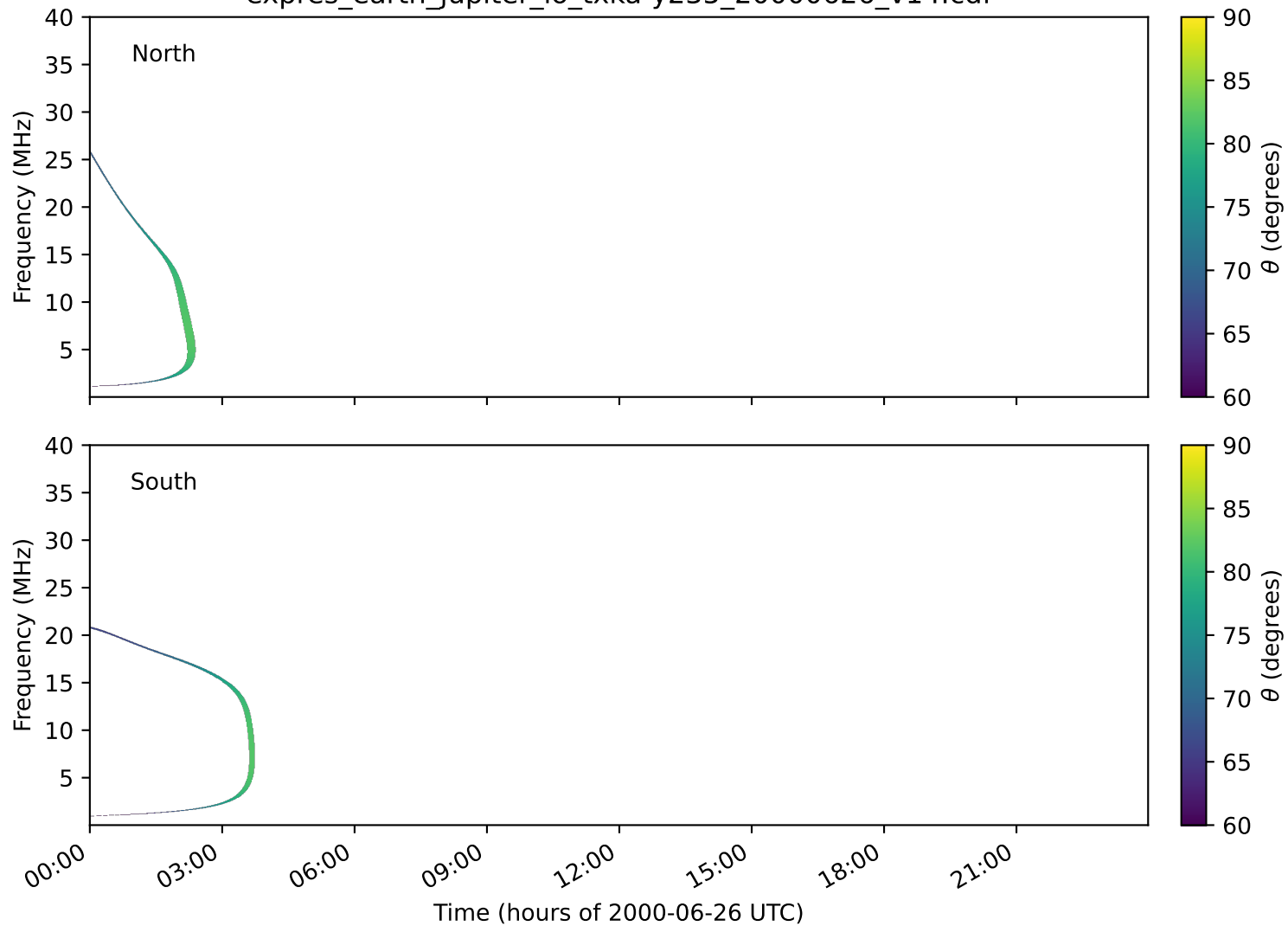
expres_earth_jupiter_io_txka-y235_20000626_v14.cdf
