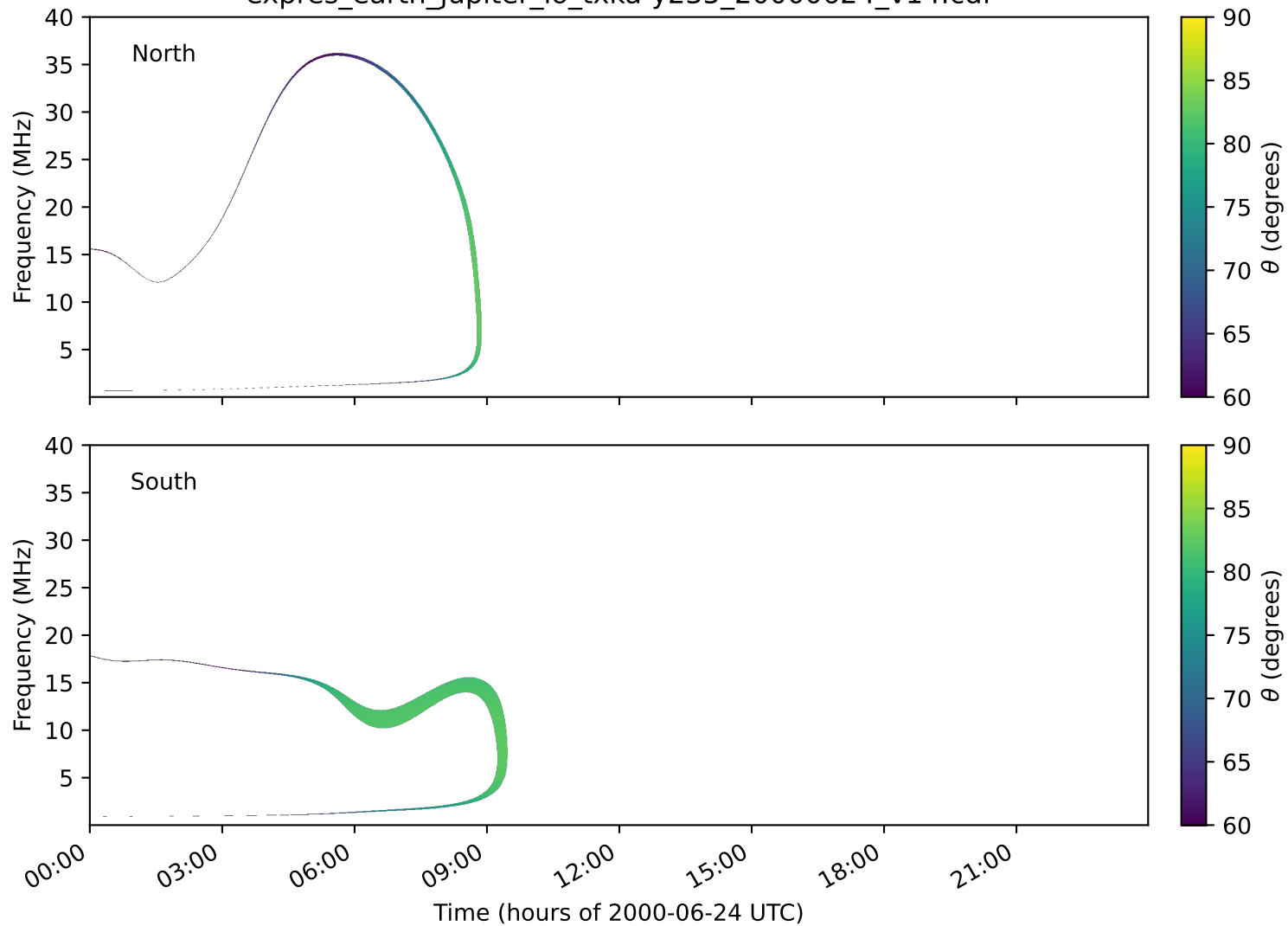
expres_earth_jupiter_io_txka-y235_20000624_v14.cdf
