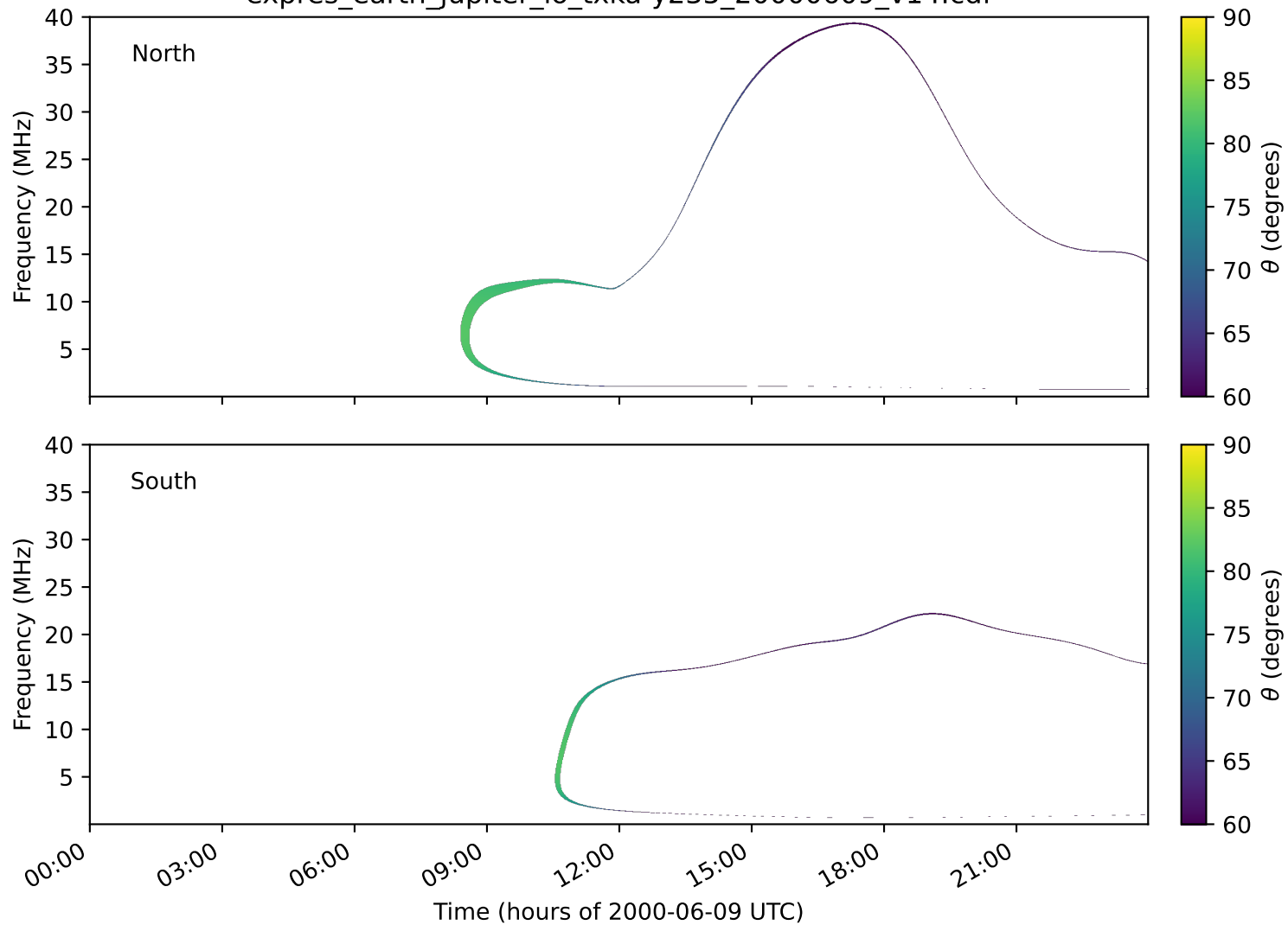
expres_earth_jupiter_io_txka-y235_20000609_v14.cdf
