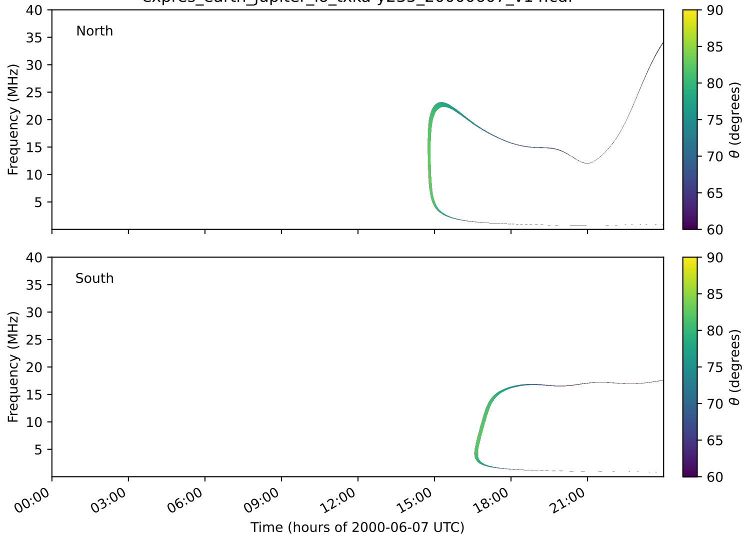
expres_earth_jupiter_io_txka-y235_20000607_v14.cdf
