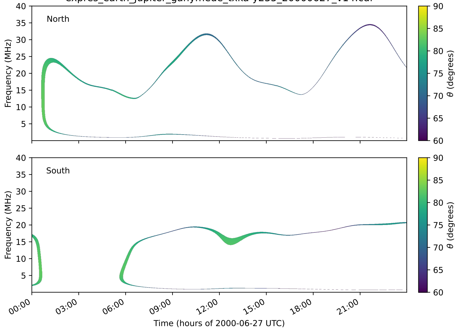
expres_earth_jupiter_ganymede_txka-y235_20000627_v14.cdf
