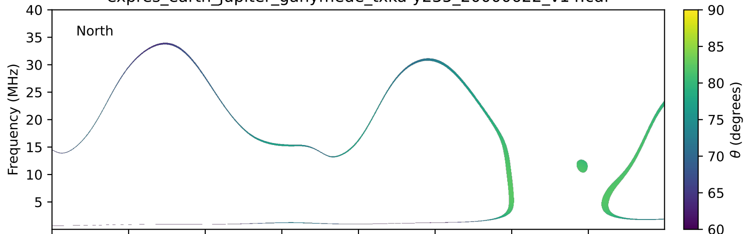
expres_earth_jupiter_ganymede_txka-y235_20000622_v14.cdf
