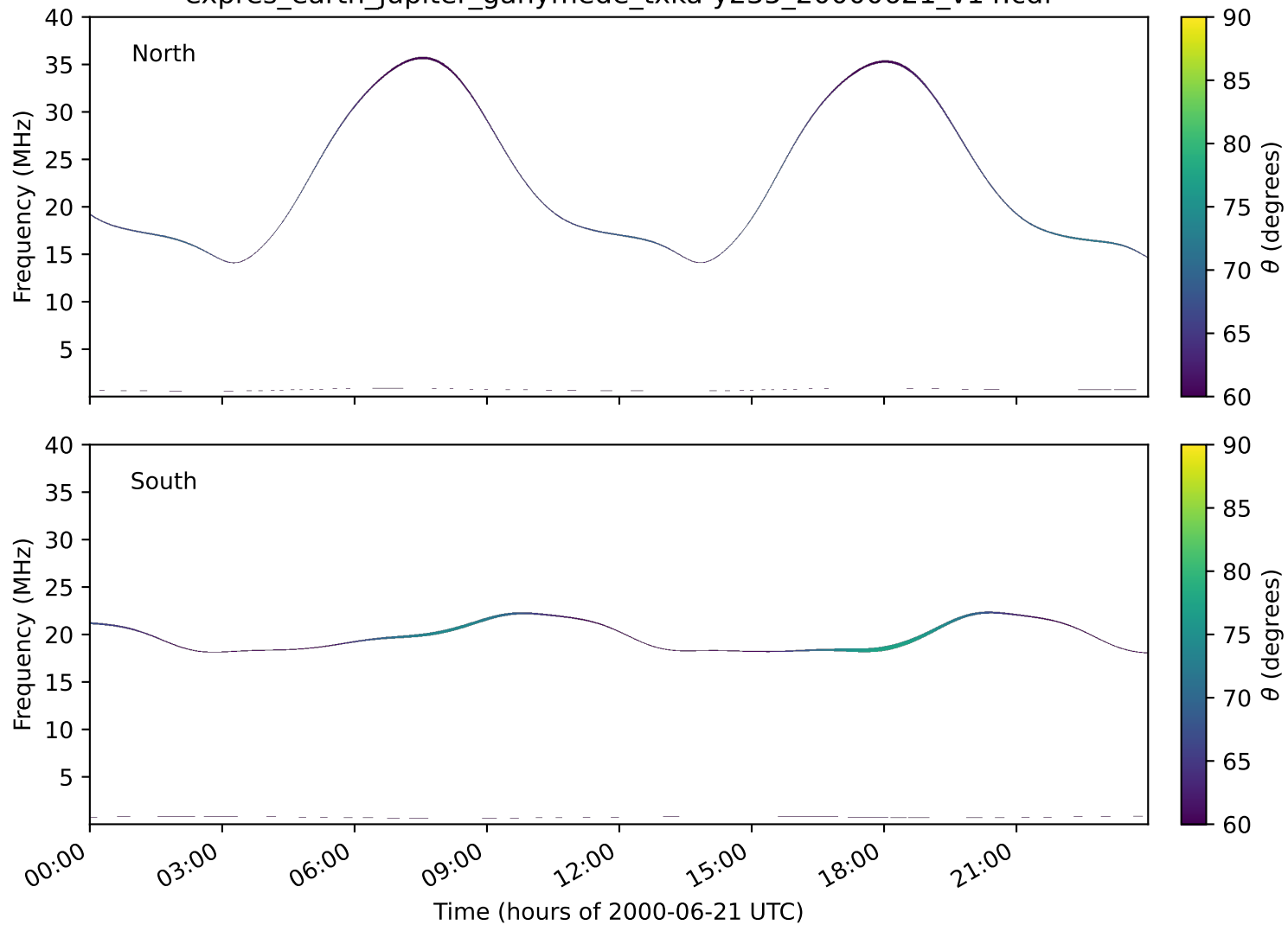
expres_earth_jupiter_ganymede_txka-y235_20000621_v14.cdf
