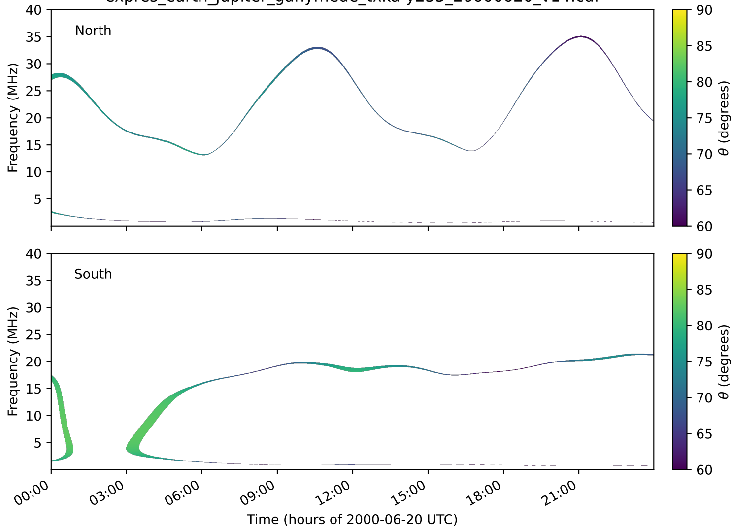
expres_earth_jupiter_ganymede_txka-y235_20000620_v14.cdf
