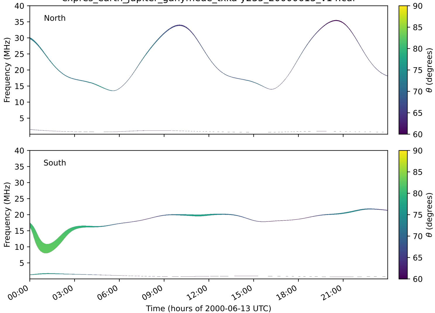
expres_earth_jupiter_ganymede_txka-y235_20000613_v14.cdf
