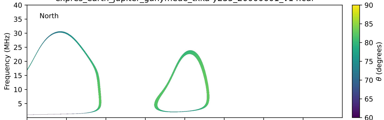
expres_earth_jupiter_ganymede_txka-y235_20000601_v14.cdf
