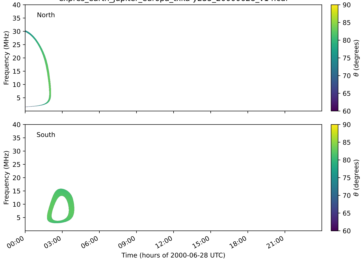
expres_earth_jupiter_europa_txka-y235_20000628_v14.cdf
