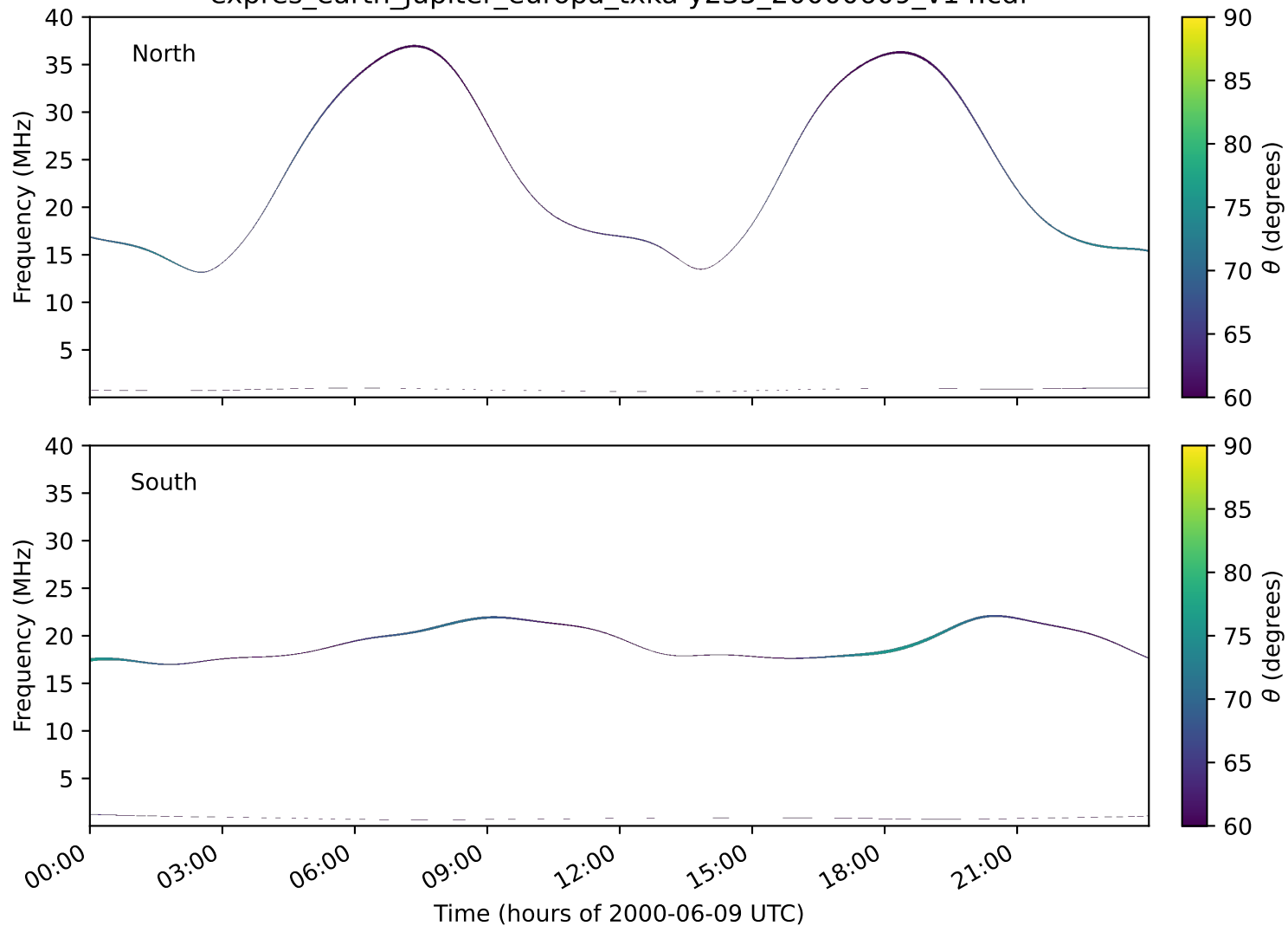
expres_earth_jupiter_europa_txka-y235_20000609_v14.cdf
