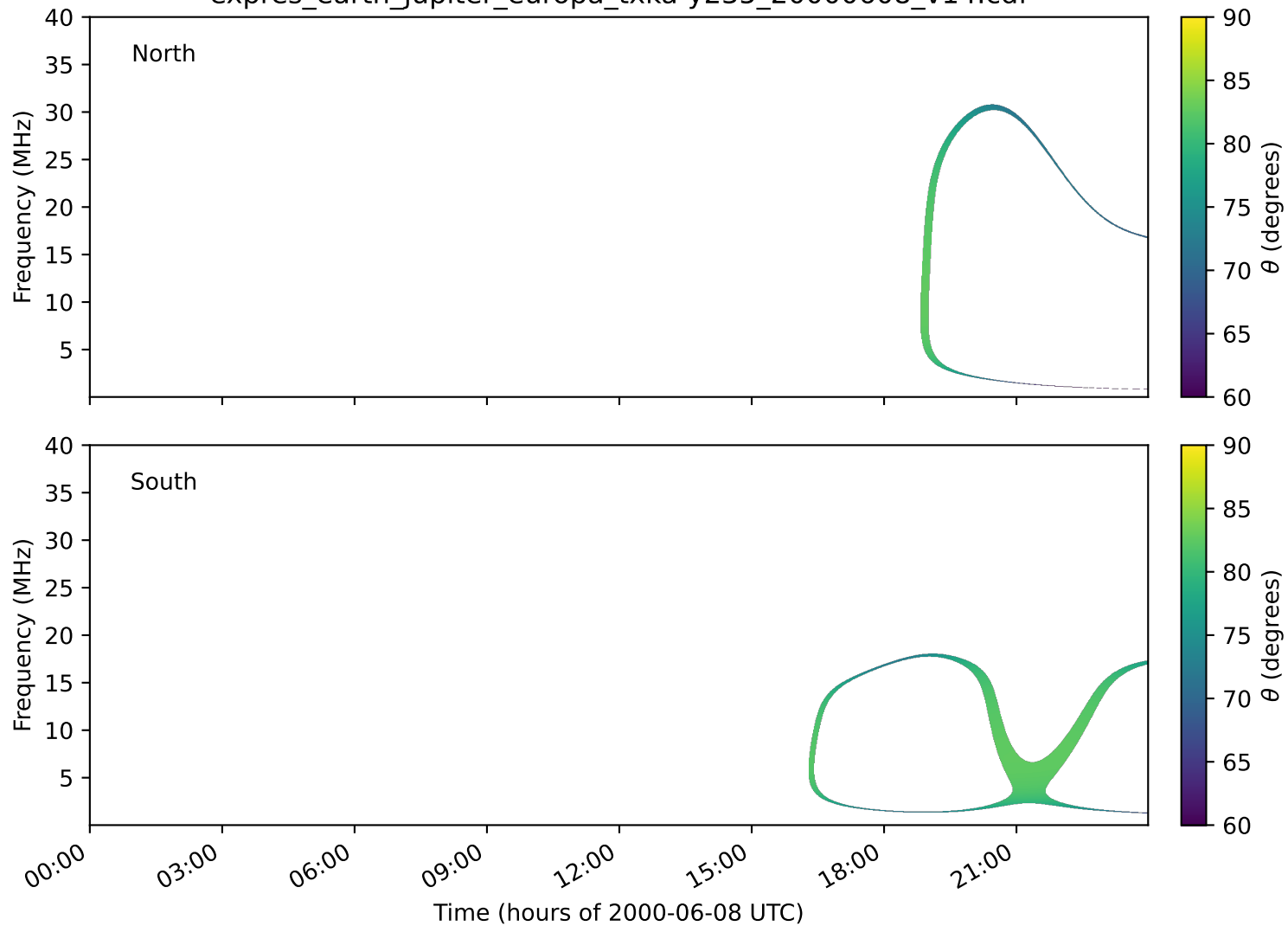
expres_earth_jupiter_europa_txka-y235_20000608_v14.cdf
