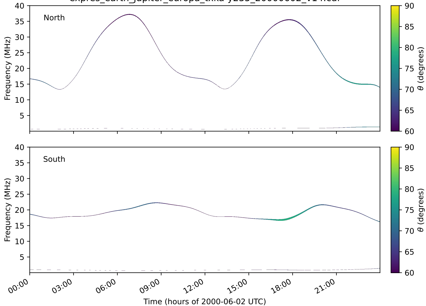
expres_earth_jupiter_europa_txka-y235_20000602_v14.cdf
