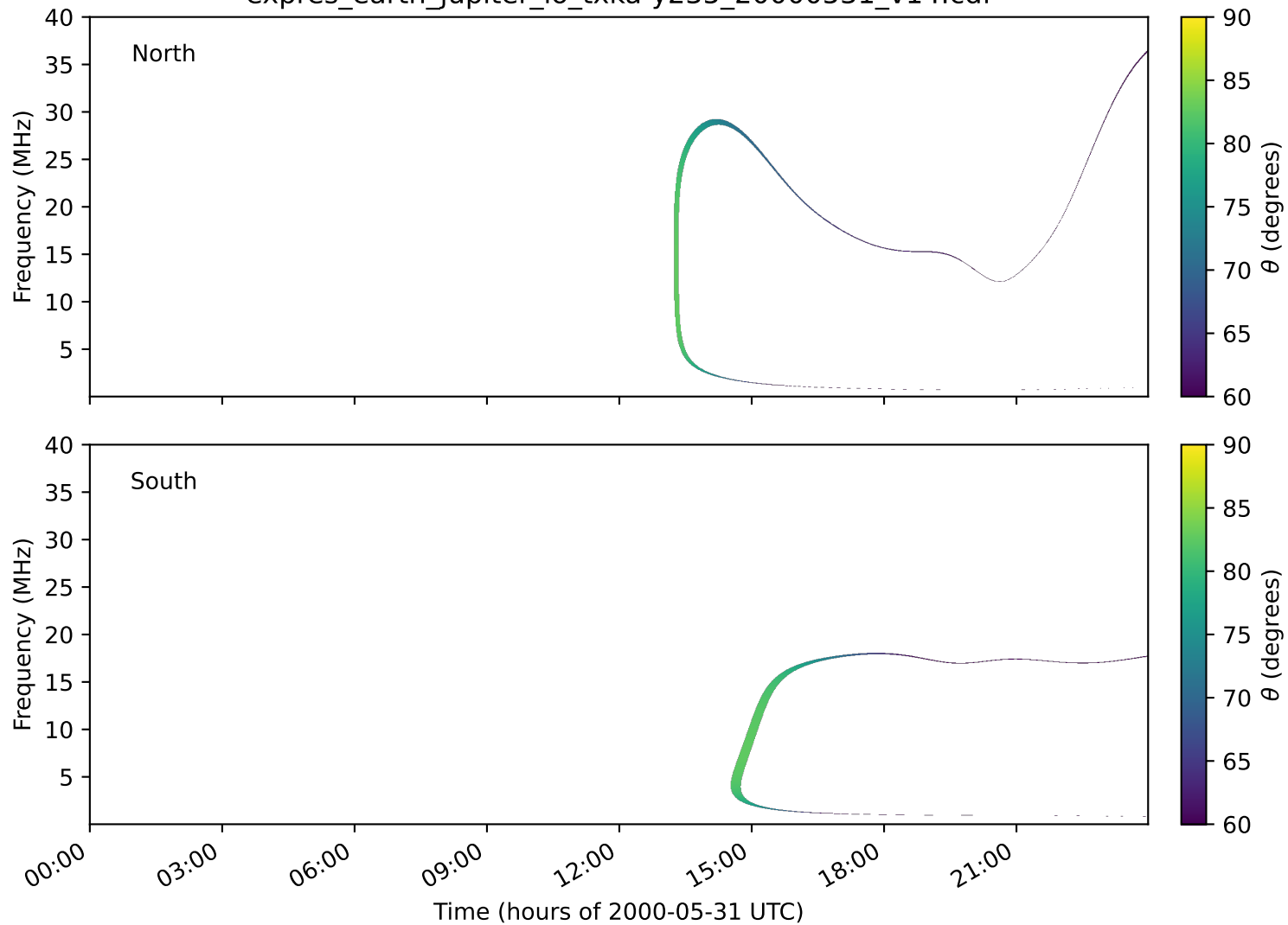
expres_earth_jupiter_io_txka-y235_20000531_v14.cdf
