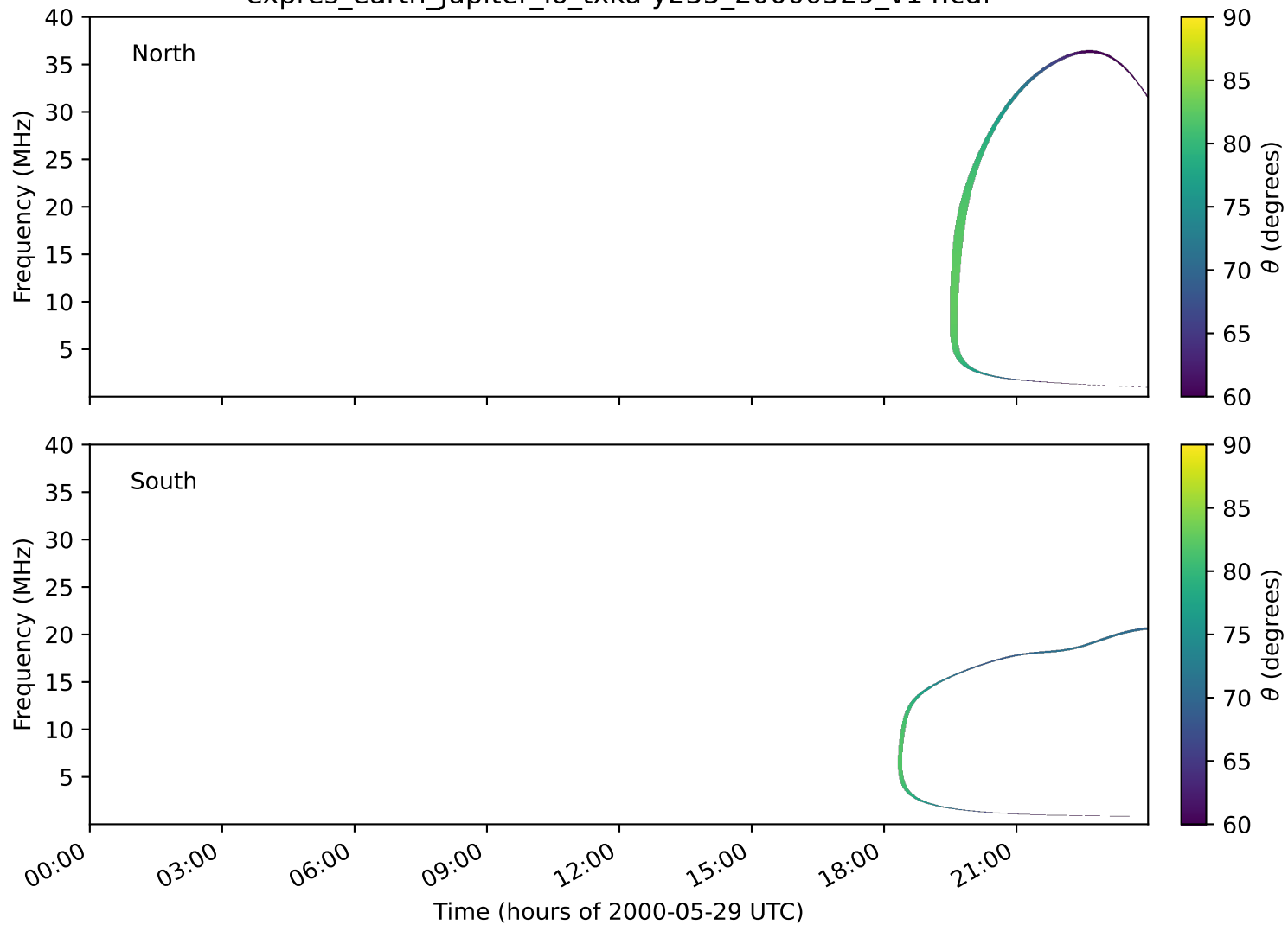
expres_earth_jupiter_io_txka-y235_20000529_v14.cdf
