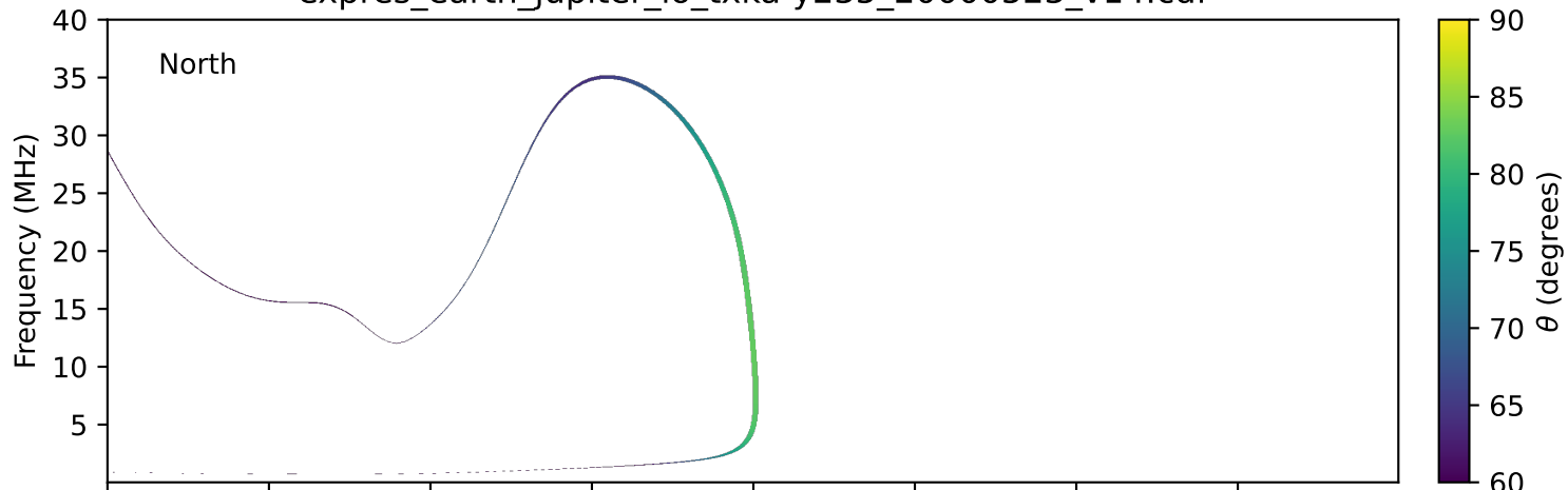
expres_earth_jupiter_io_txka-y235_20000523_v14.cdf
