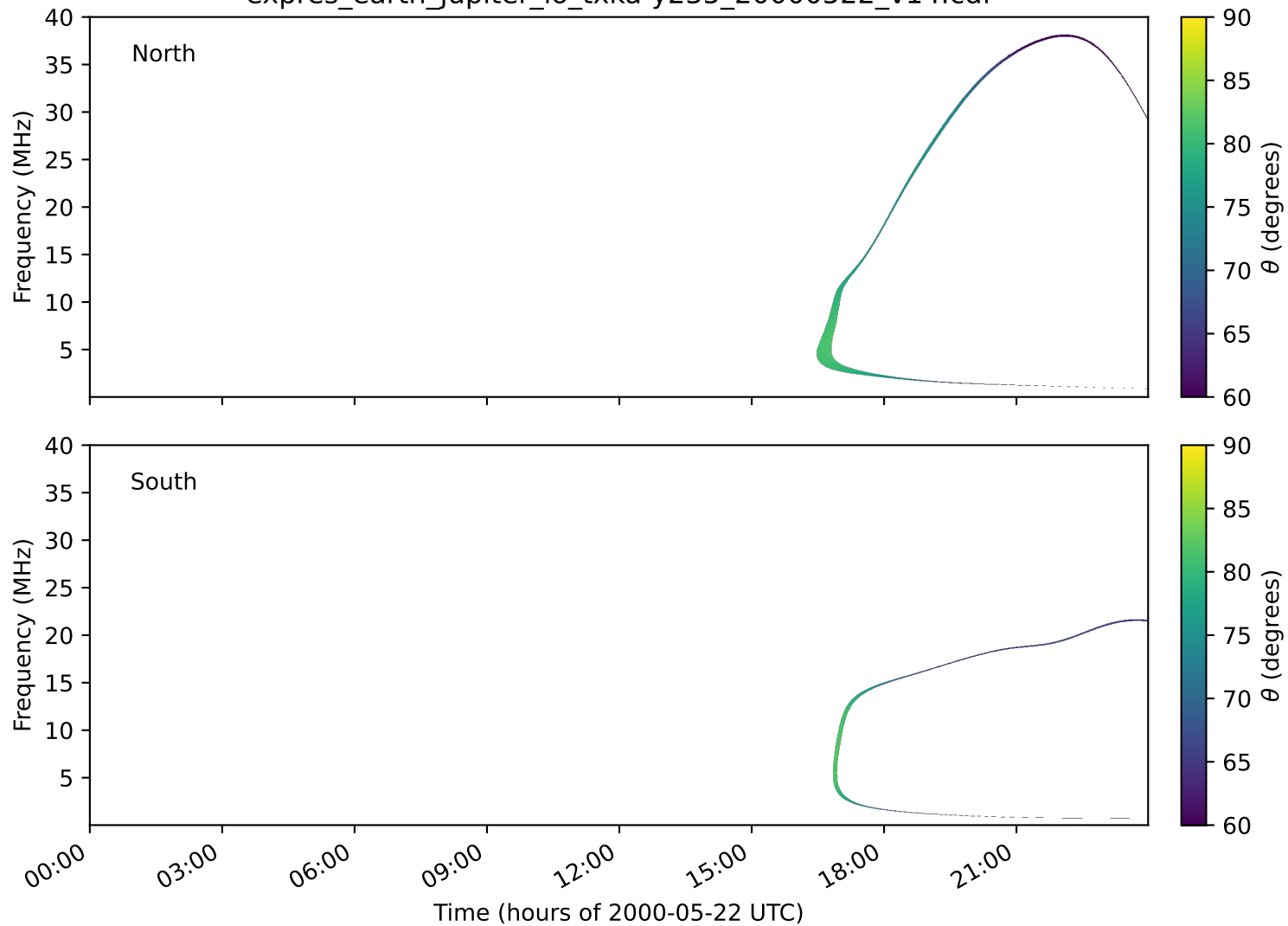
expres_earth_jupiter_io_txka-y235_20000522_v14.cdf
