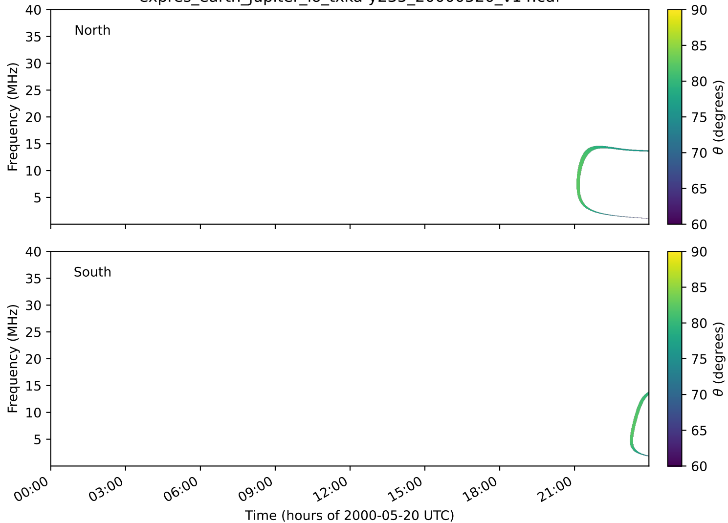
expres_earth_jupiter_io_txka-y235_20000520_v14.cdf
