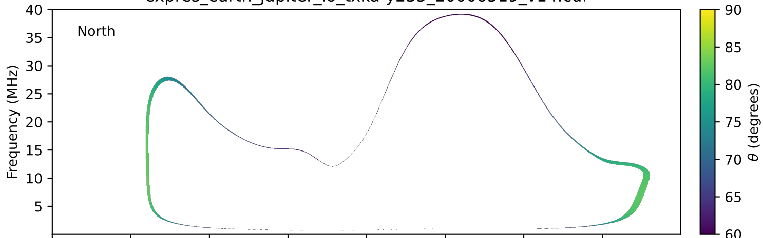
expres_earth_jupiter_io_txka-y235_20000519_v14.cdf
