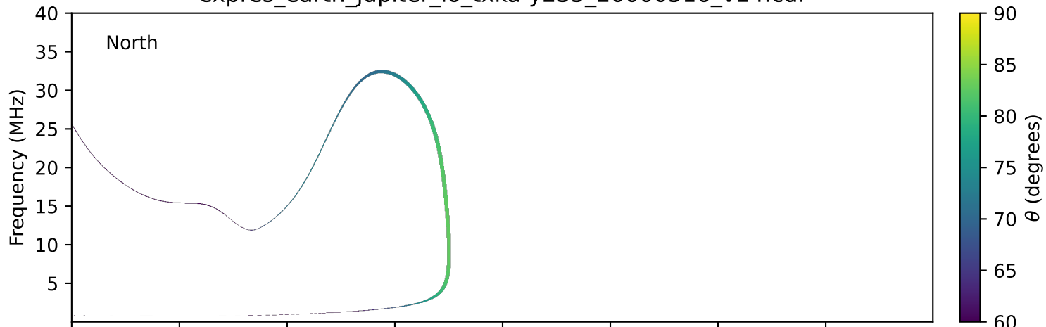
expres_earth_jupiter_io_txka-y235_20000516_v14.cdf
