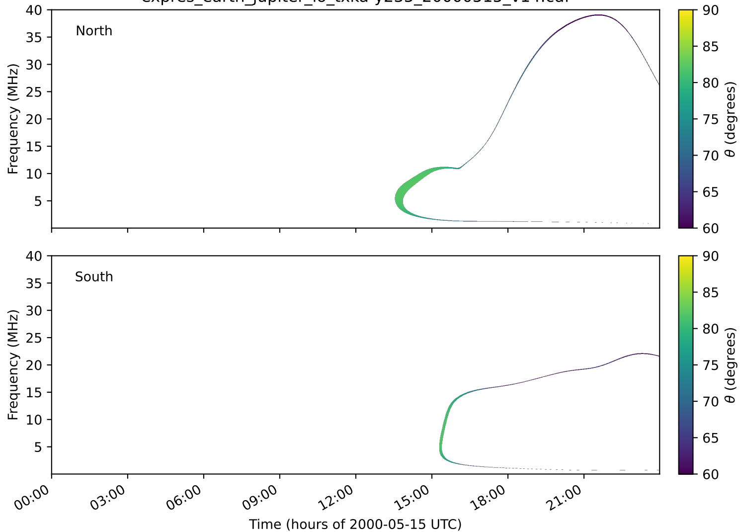
expres_earth_jupiter_io_txka-y235_20000515_v14.cdf
