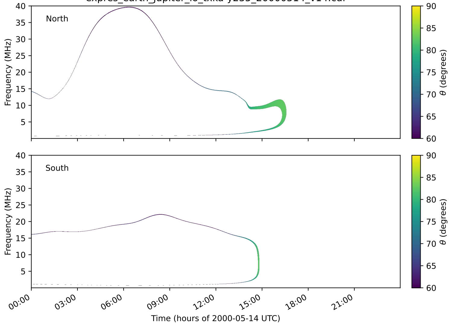
expres_earth_jupiter_io_txka-y235_20000514_v14.cdf
