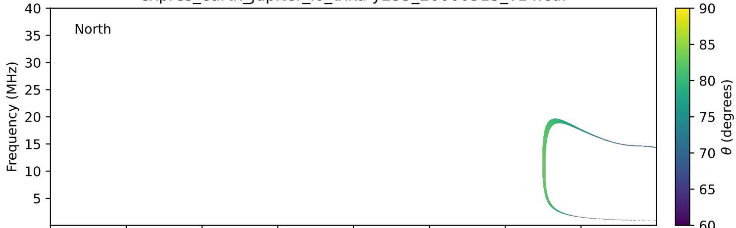
expres_earth_jupiter_io_txka-y235_20000513_v14.cdf
