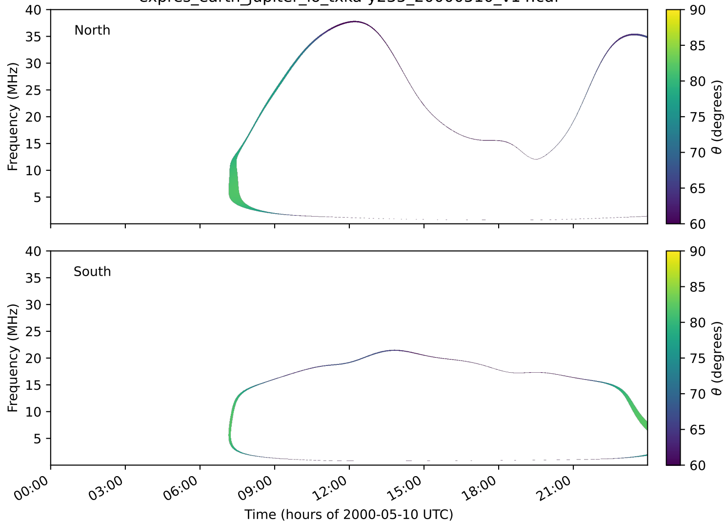
expres_earth_jupiter_io_txka-y235_20000510_v14.cdf
