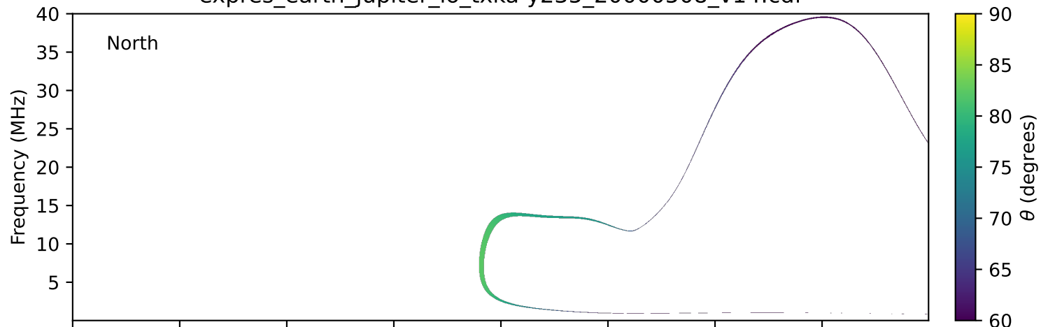
expres_earth_jupiter_io_txka-y235_20000508_v14.cdf
