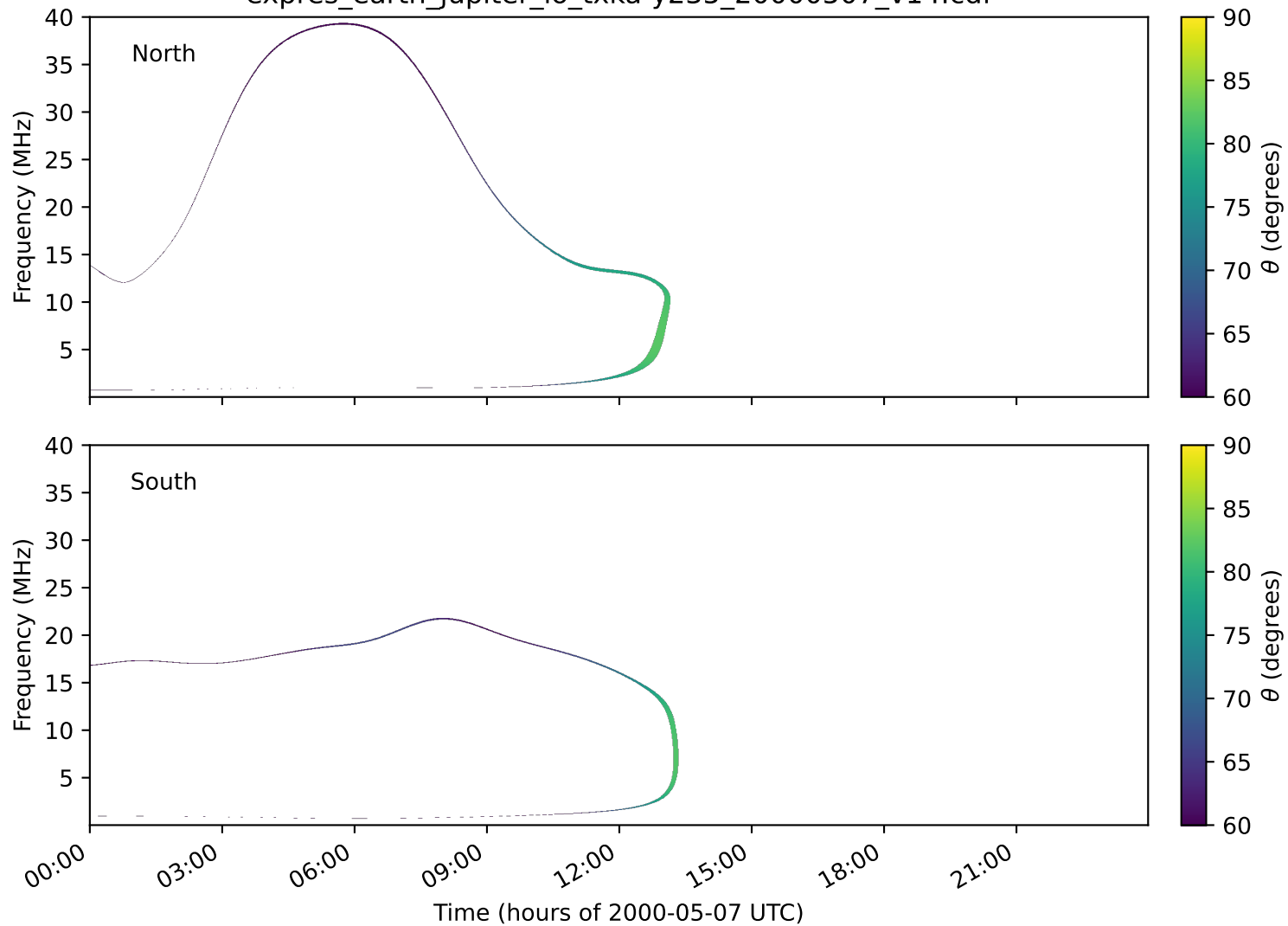
expres_earth_jupiter_io_txka-y235_20000507_v14.cdf
