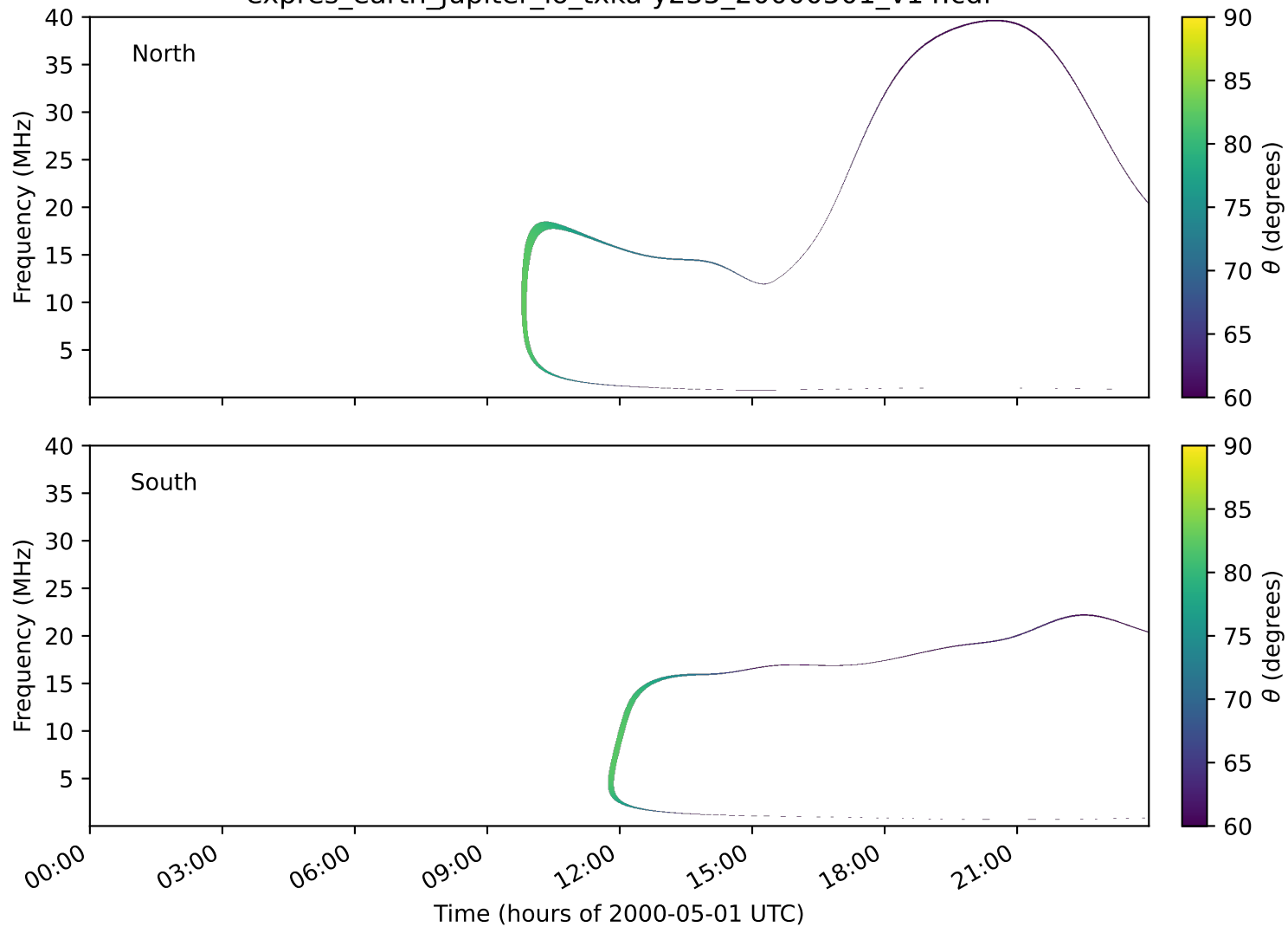
expres_earth_jupiter_io_txka-y235_20000501_v14.cdf
