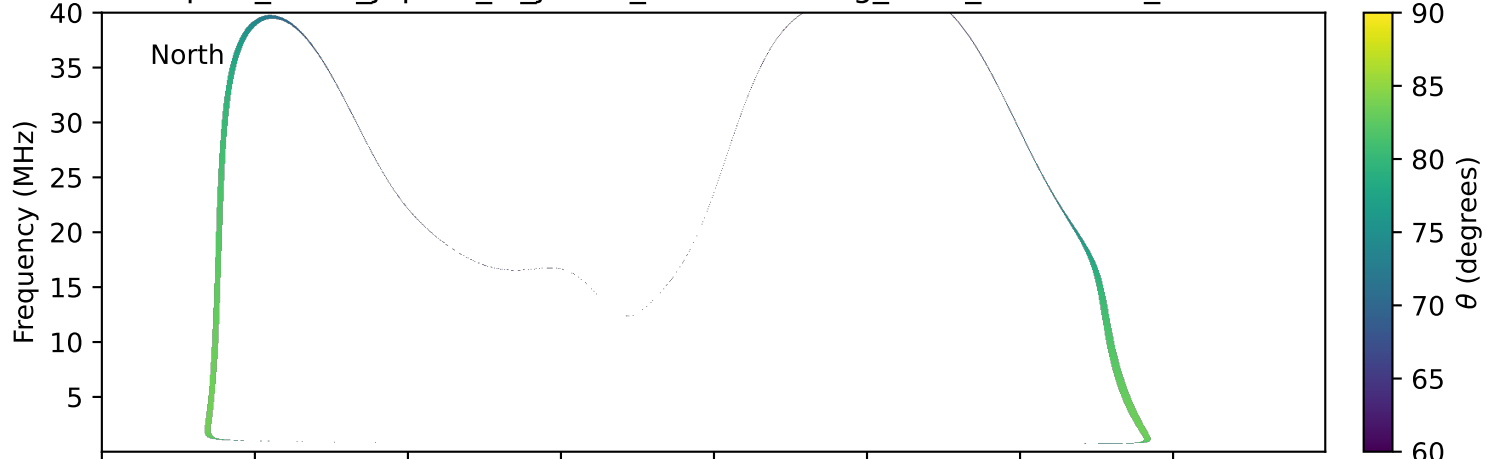
expres_earth_jupiter_io_jrm33_lossc-wid1deg_3kev_20000512_v11.cdf
