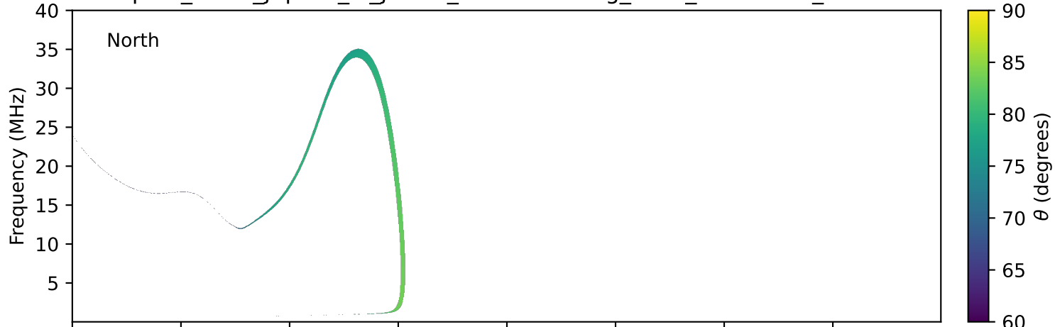
expres_earth_jupiter_io_jrm33_lossc-wid1deg_3kev_20000509_v11.cdf
