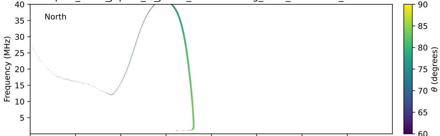
expres_earth_jupiter_io_jrm09_lossc-wid1deg_3kev_20000516_v11.cdf
