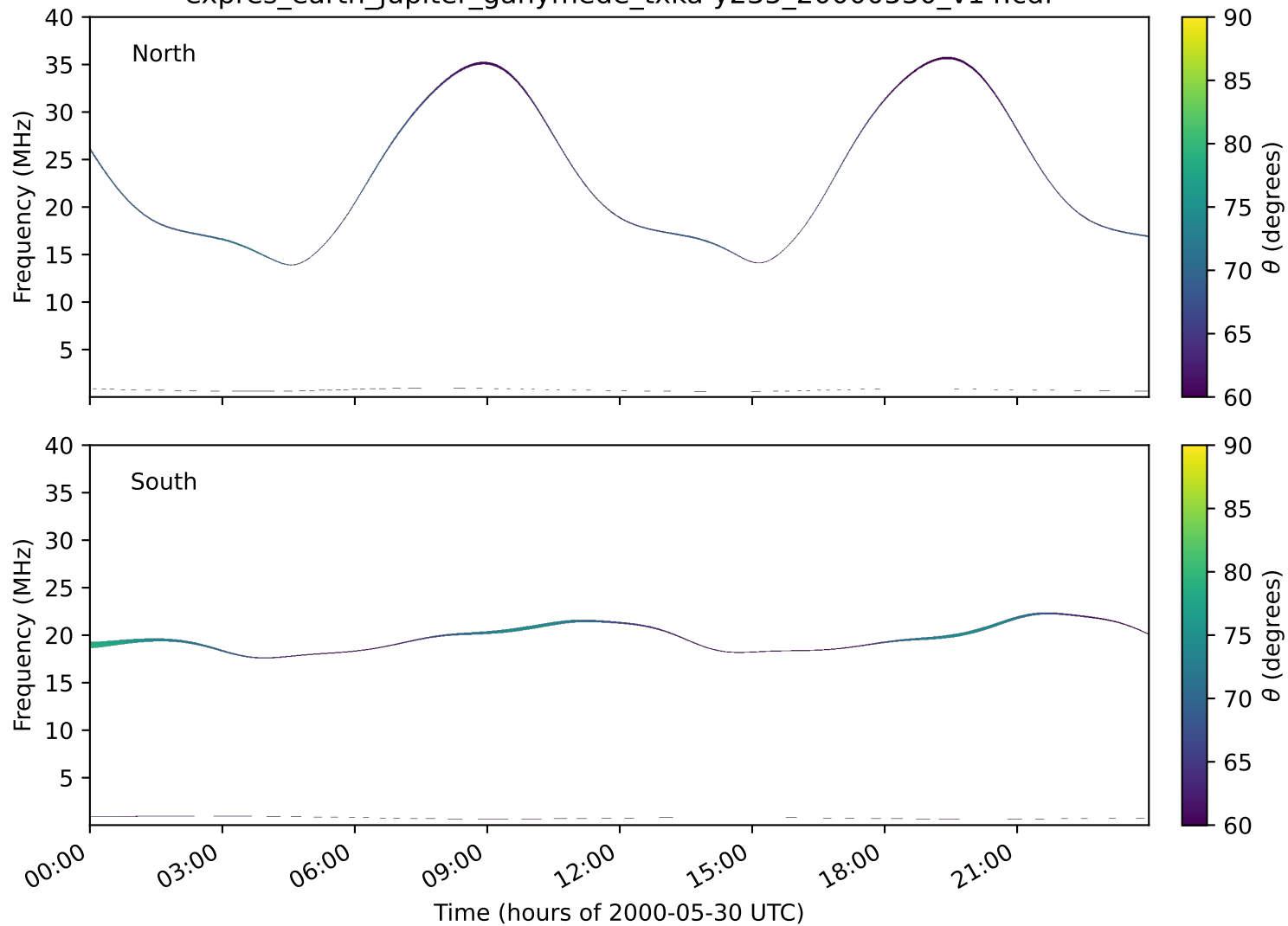
expres_earth_jupiter_ganymede_txka-y235_20000530_v14.cdf
