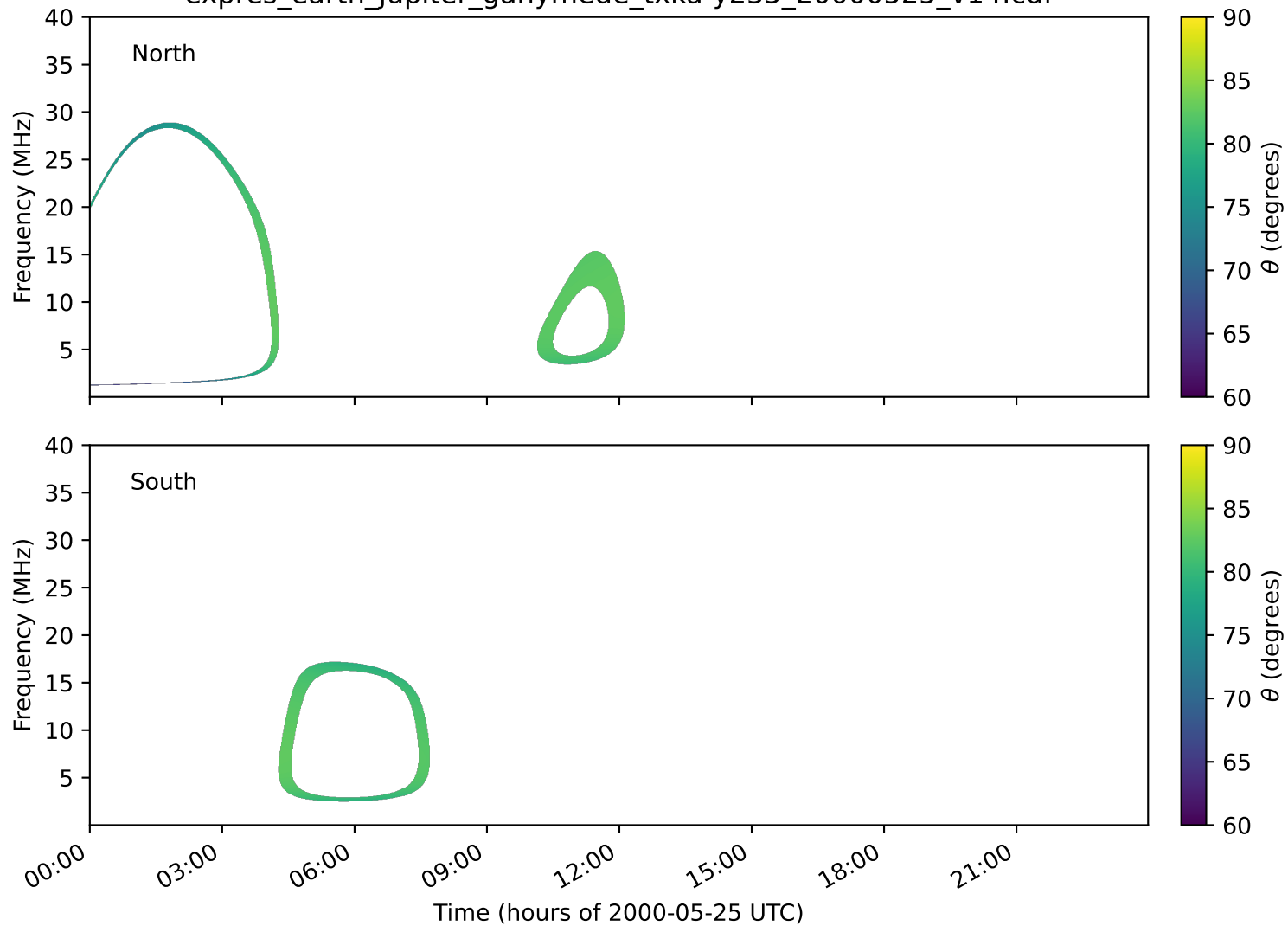
expres_earth_jupiter_ganymede_txka-y235_20000525_v14.cdf
