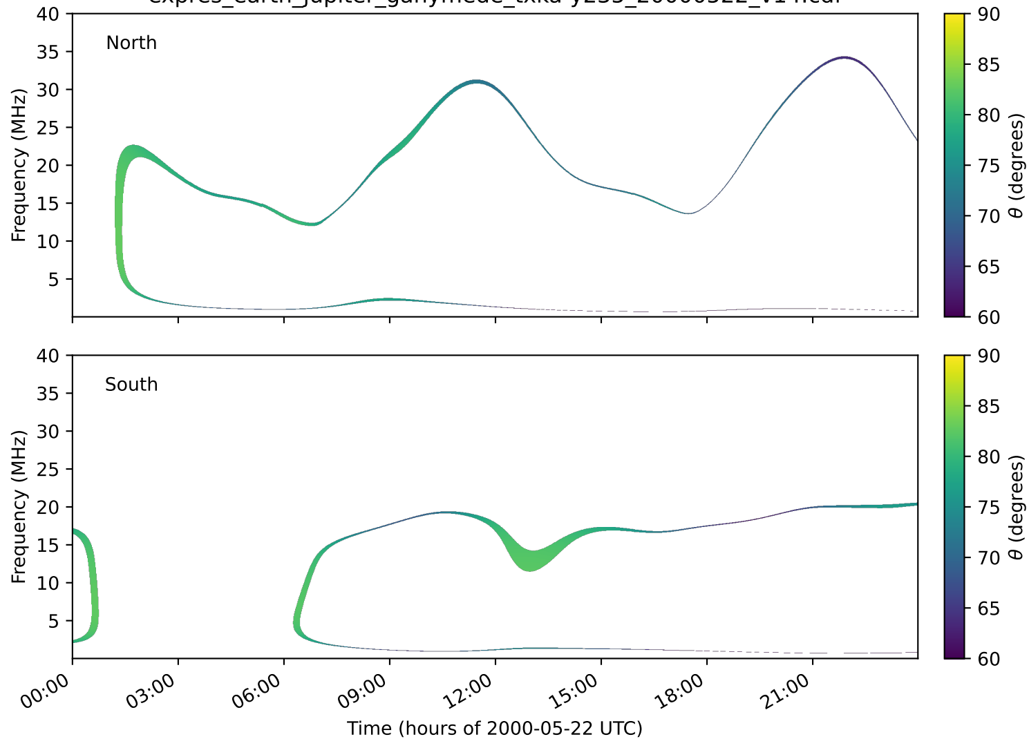
expres_earth_jupiter_ganymede_txka-y235_20000522_v14.cdf
