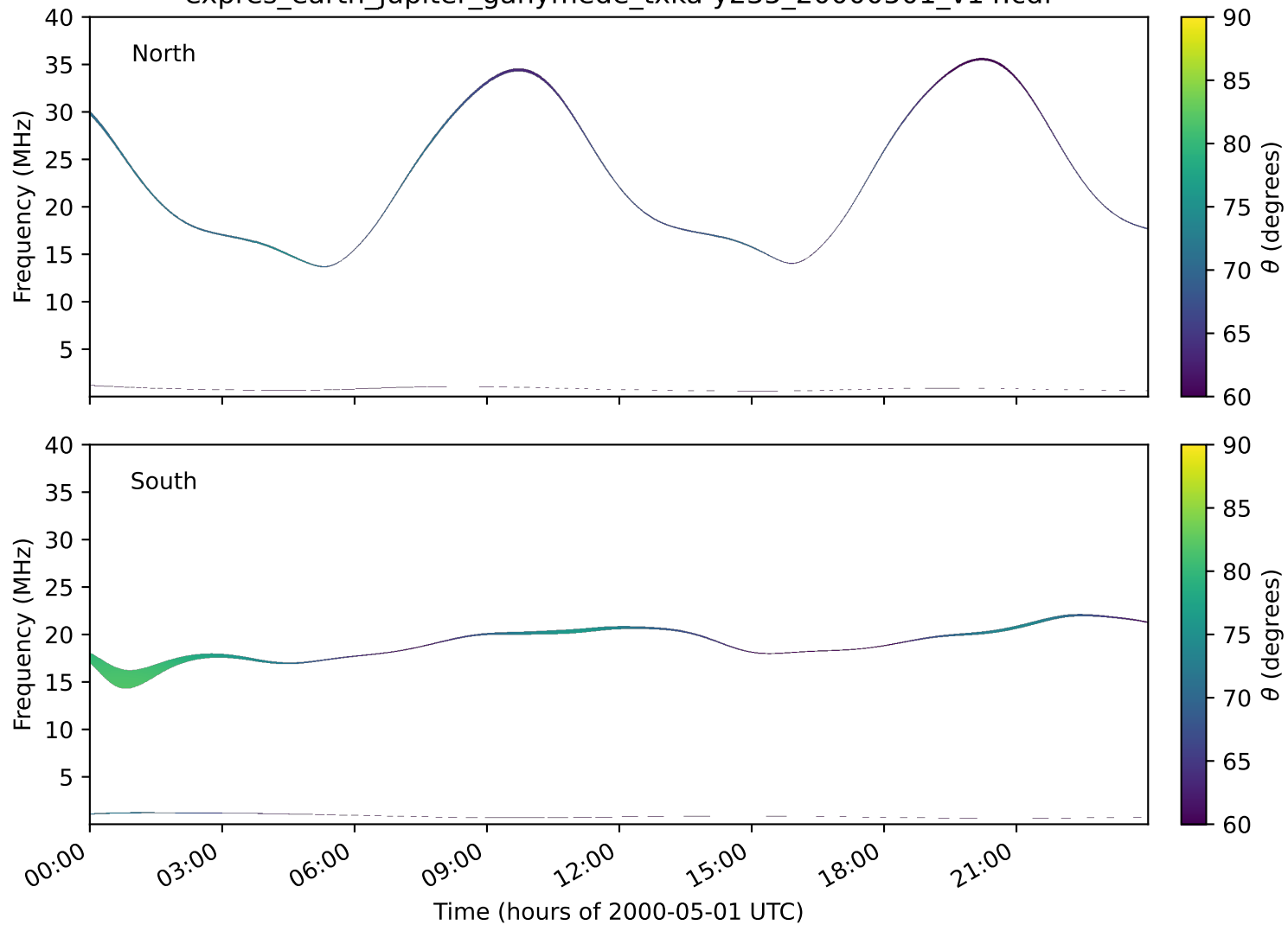
expres_earth_jupiter_ganymede_txka-y235_20000501_v14.cdf
