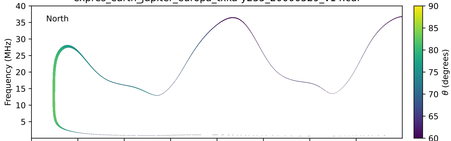
expres_earth_jupiter_europa_txka-y235_20000529_v14.cdf
